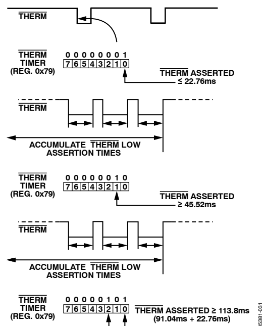
Figure 28. Understanding the THERM Timer
